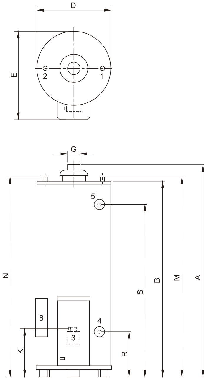
Figure 3 - Dimensions
